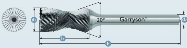
Radius + Cylinder with end cut
